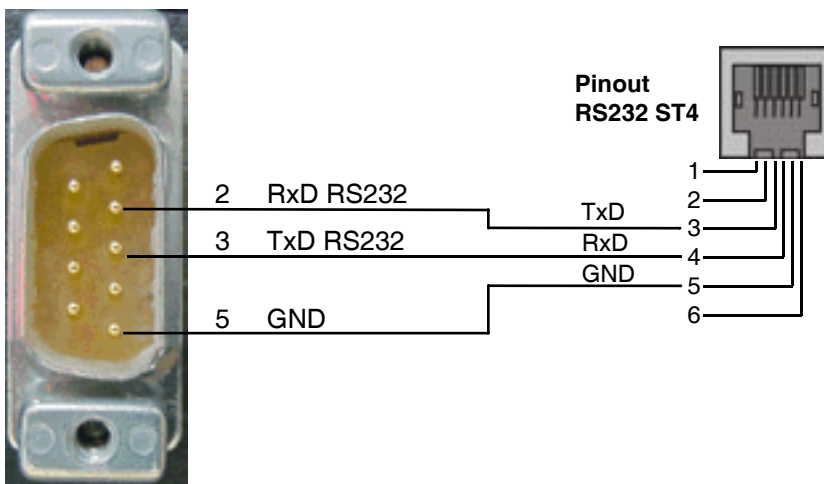
RS232 9-pol Stecker am Computer
