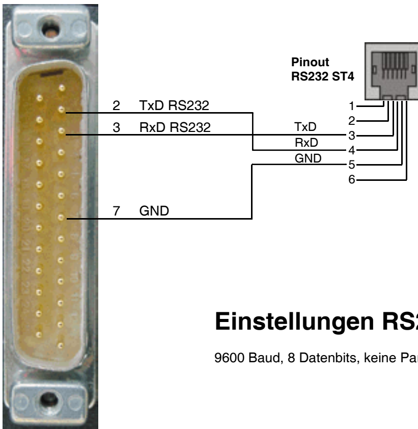
RS232 25-pol Stecker am Computer
